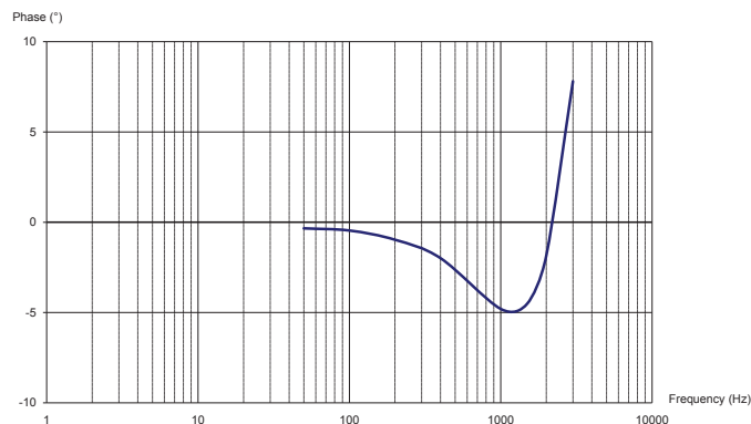
Curve B: Typical Phase Error vs Frequency
